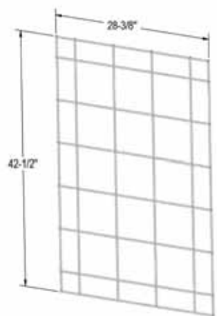
Modular Grid-Vertical
